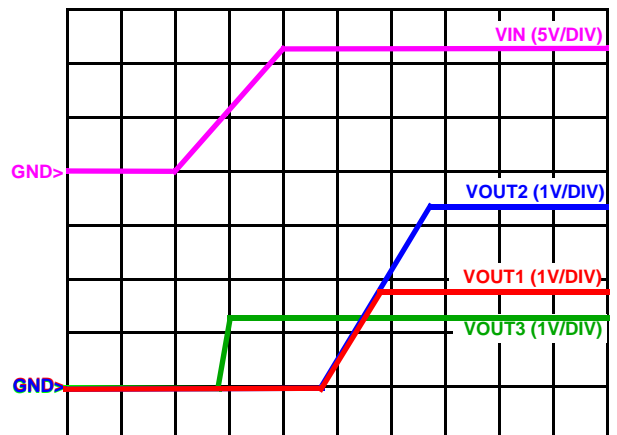
FIGURE 7. OUTPUT VOLTAGES
