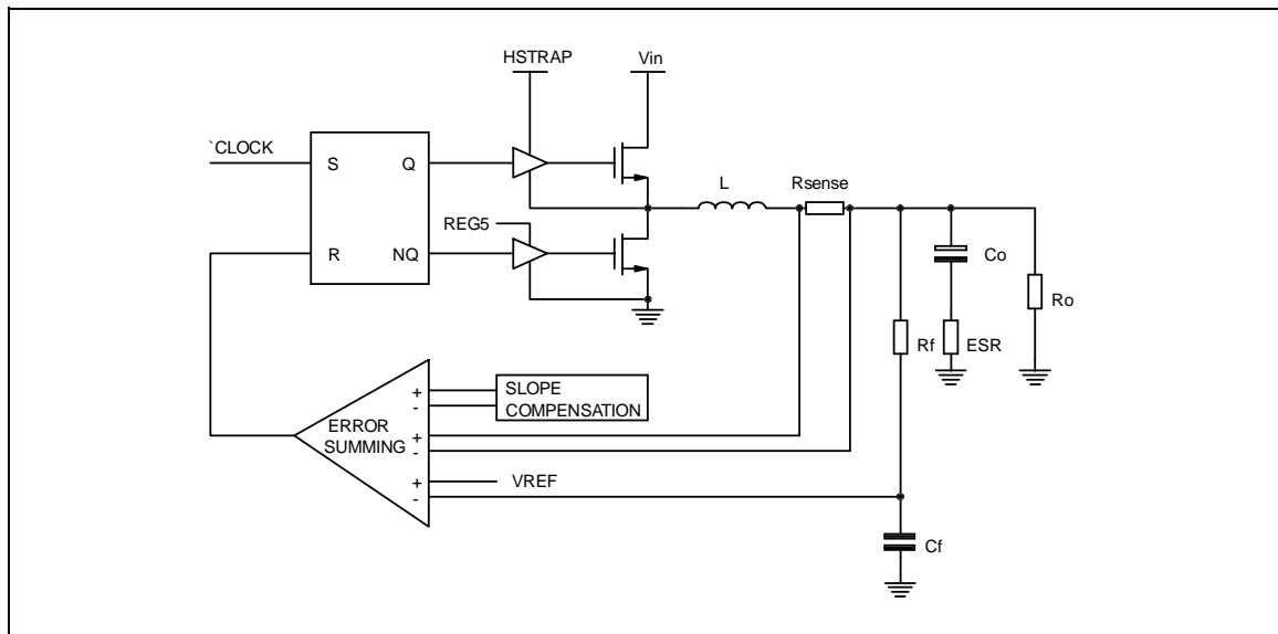
Figure 3. Control loop.
