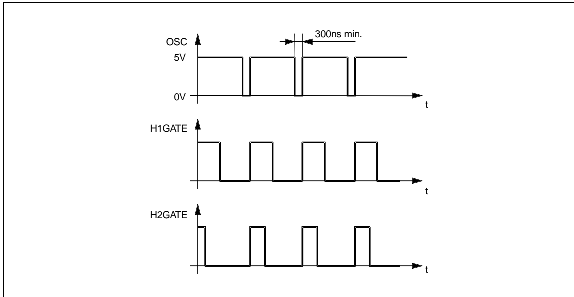
Figure 2. Synchronization signal and operation
