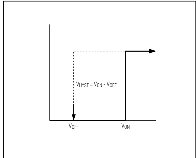
Figure 3. MAX5068 Hysteresis
