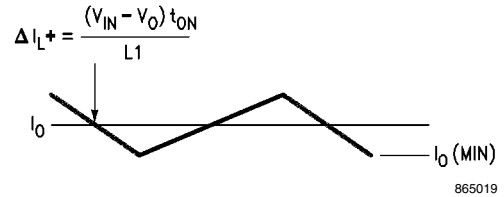
FIGURE 14. Inductor Current Slope in Step-Down Regulator
