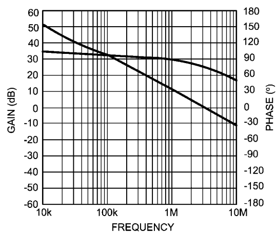
Feedback Amplifier Gain/Phase
