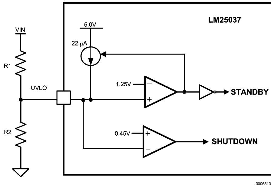
FIGURE 14. Basic UVLO Configuration
