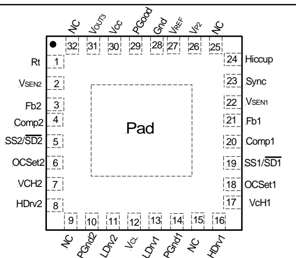
32-Lead MLPQ 5mmx5mm (M)
