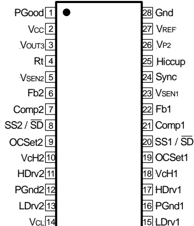
28-PIN TSSOP (F)
