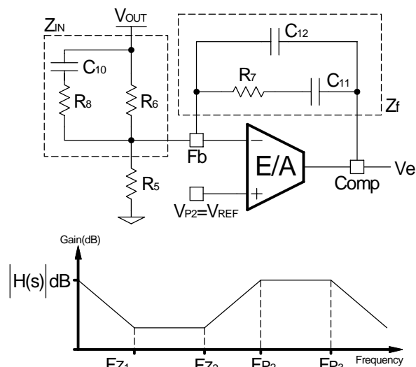
Figure 16- Compensation network with local feedback and its asymptotic gain plot.
