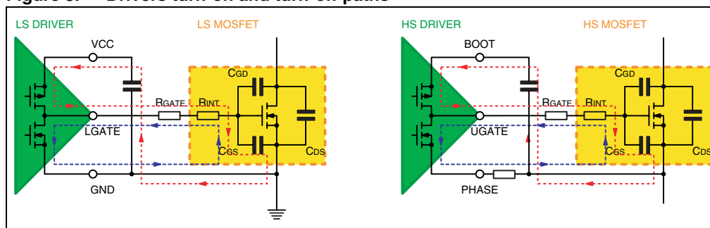
Figure 8. Drivers turn-on and turn-off paths
