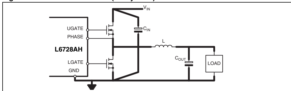
Figure 7. Power connections (heavy lines)
