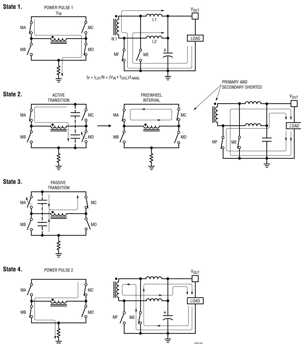
Figure 1. ZVS Operation
