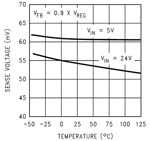
Current Limit Sense Voltage
