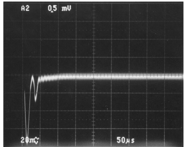
Transient Response with Output Capacitor Halved
