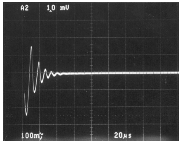
Transient Response with Only 4.7 \mu F Output Cap
