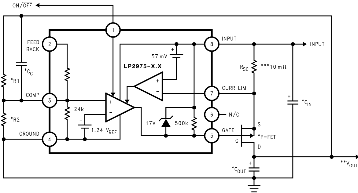
Adjustable Voltage 5A LDO Regulator
