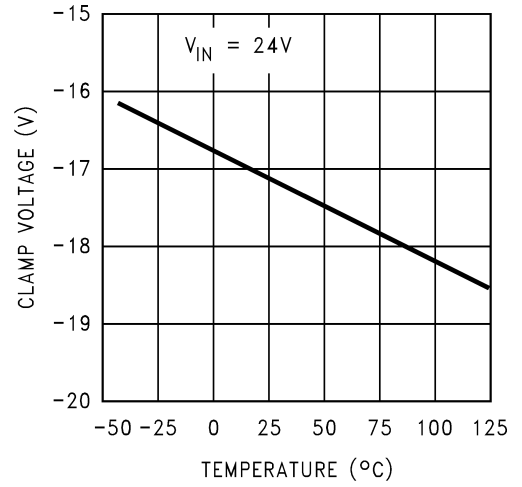
V_{IN} Referred Gate Clamp Voltage
