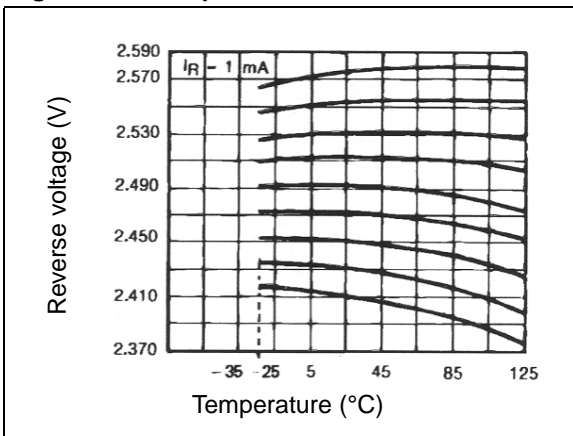
Figure 8. Temperature drift
