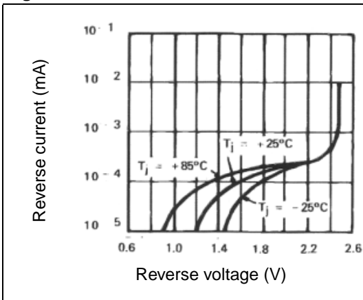
Figure 8. Temperature drift
