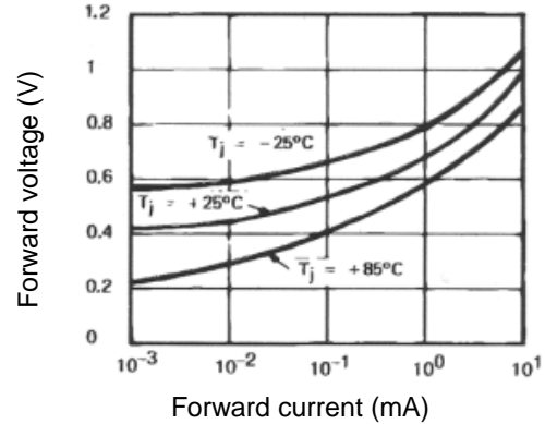
Figure 7. Forward characteristics
