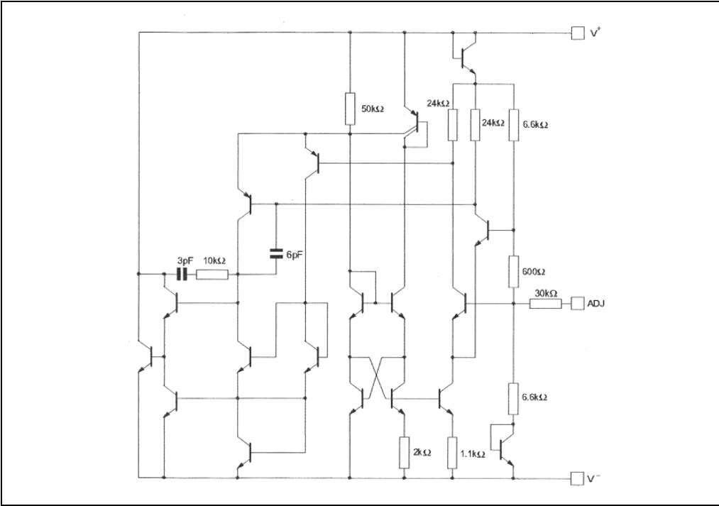
Figure 1. Schematic diagram
