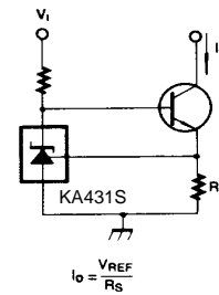
Figure 17. Constant-Current Sink
