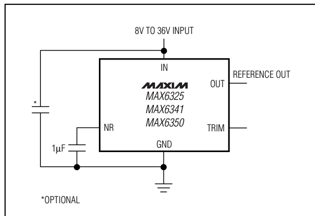
Figure 2. Noise-Reduction Capacitor
