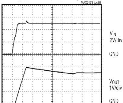
TURN-ON TRANSIENT ( V_{OUT} = 2.5V , C_{OUT} = 1\mu F )
