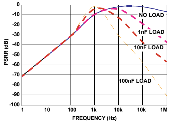
FIGURE 22. PSSR vs CAP LOAD
