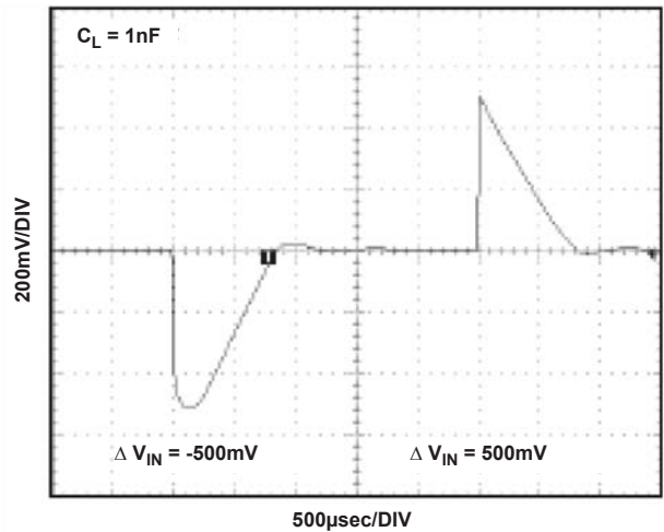
FIGURE 9. LINE TRANSIENT RESPONSE, 0.001µF LOAD CAPACITANCE
