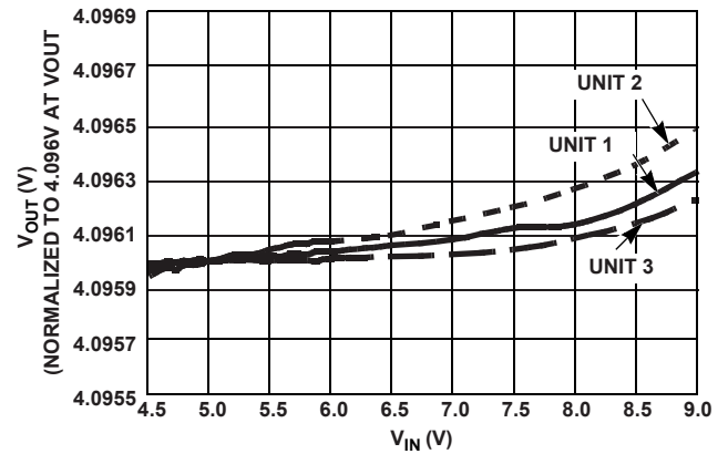
FIGURE 6. LINE REGULATION (3 UNITS)
