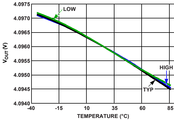
FIGURE 5. V_{OUT} vs TEMPERATURE NORMALIZED TO +25^\circ C (3 UNITS)
