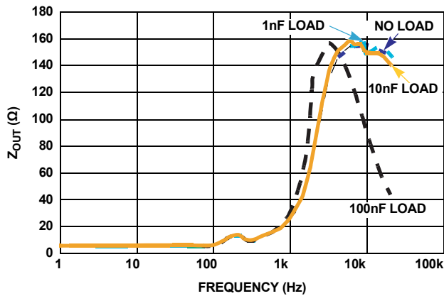
FIGURE 28. Z_{OUT} vs FREQUENCY
