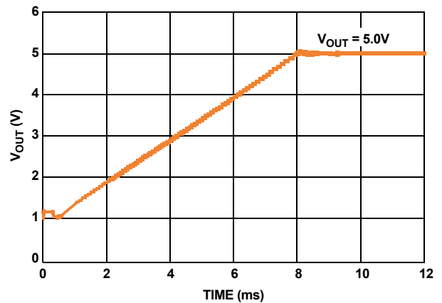
FIGURE 31. TURN-ON TIME
