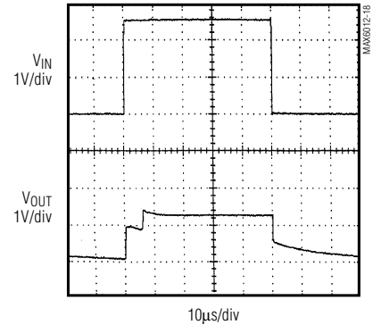
MAX6012 TURN-ON TRANSIENT
