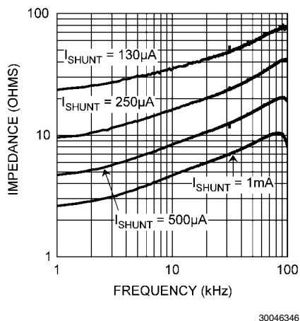
FIGURE 2. Reverse Dynamic Impedance vs I_{OUT}
