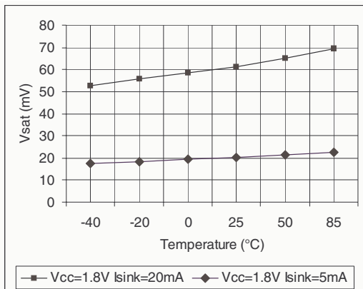
Figure 6. V_{SAT} vs. temperature
