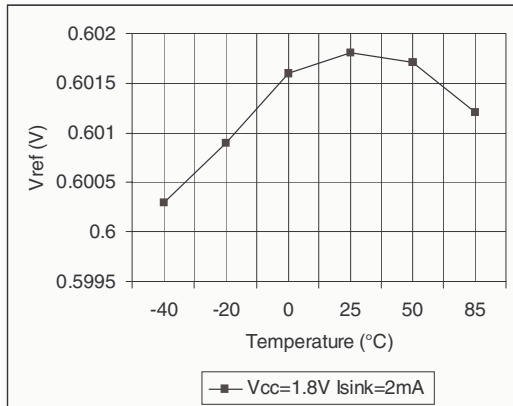
Figure 2. V_{ref} vs. temperature
