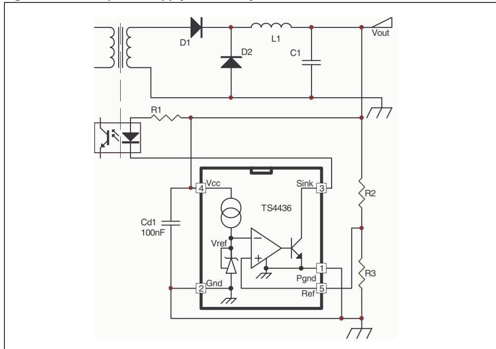
Figure 1. SMPS power supply: secondary side
