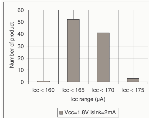
Figure 5. I_{CC} at 25°C
