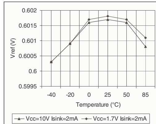
Figure 3. V_{ref} vs. temperature
