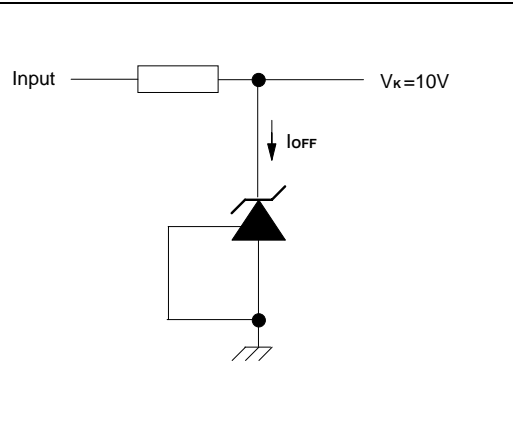
Figure 8. Test circuit for off-state current measurement
