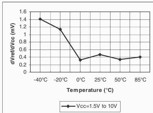
Figure 4. dVref/dVcc vs. temp. Isink=2mA
