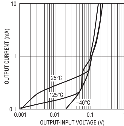
2.5V Minimum V_{OUT}-V_{IN} Differential (Sinking)
