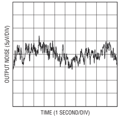
5V Low Frequency 0.1Hz to 10Hz Transient Noise
