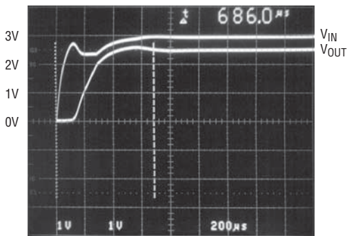
Figure 1. Turn-On Characteristics of LT1790-2.5
