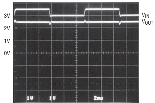
Figure 2. Output Response to 0.5V Ripple on V_{IN}
