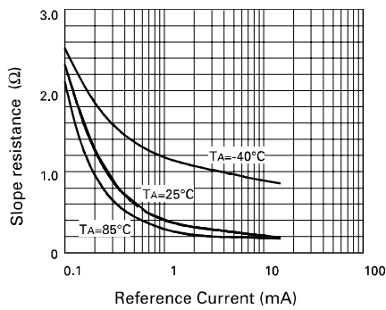
Slope Resistance v Current
