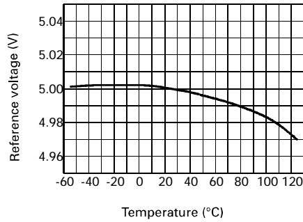
Temperature Drift
