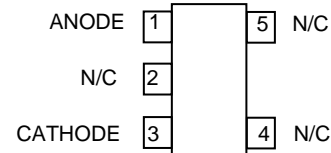
LM4041_H5 (SC70-5)
