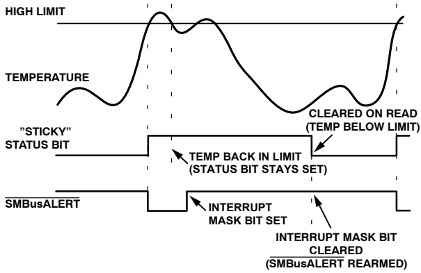
Figure 31. Handling SMBusALERT
