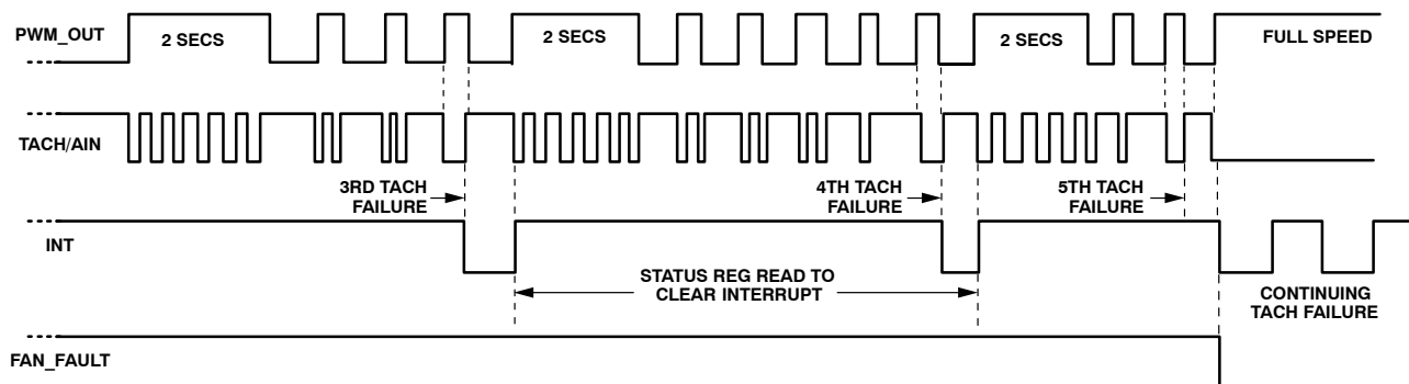
Figure 38. Operation of \overline{\text{FAN\_FAULT}} and Interrupt Pins
