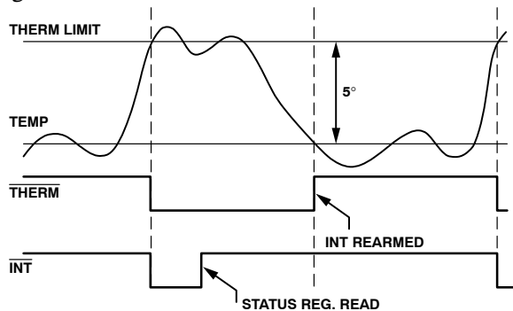
Figure 20. Operation of \overline{\text{THERM}} and \overline{\text{INT}} Signals
