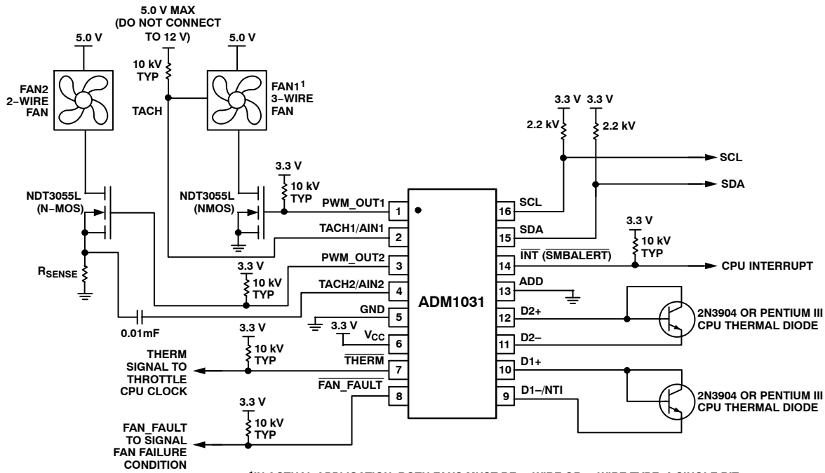
Figure 39. Typical Application Circuit
