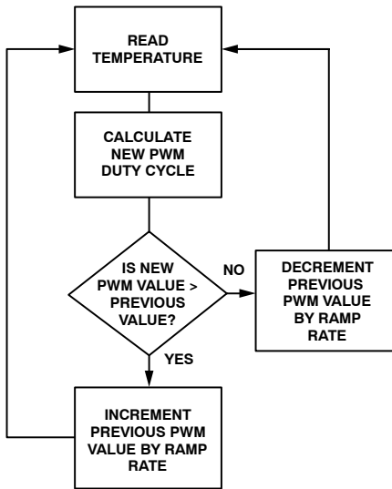
Figure 28. Filtered Mode Algorithm
