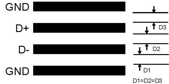
FIGURE 8. Ideal Diode Trace Layout
