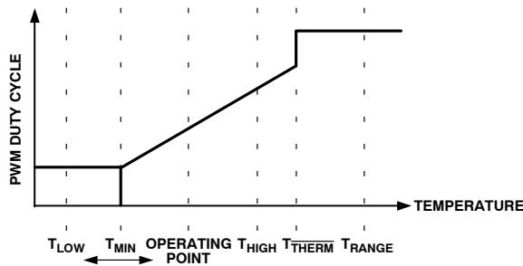
Figure 66. Dynamic T_{MIN} Control Loop
