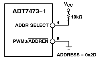
Figure 15. SMBus Address = 0x2D (Pin 4 = 1)
