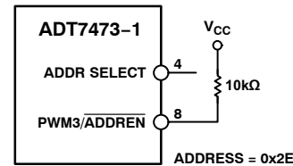
Figure 13. Default SMBus Address = 0x2E
