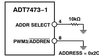
Figure 14. SMBus Address = 0x2C (Pin4 = 0)
