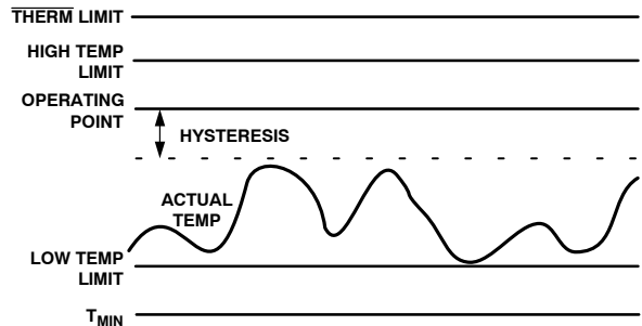
Figure 70. Temperature Between Operating Point and Low Temperature Limit
