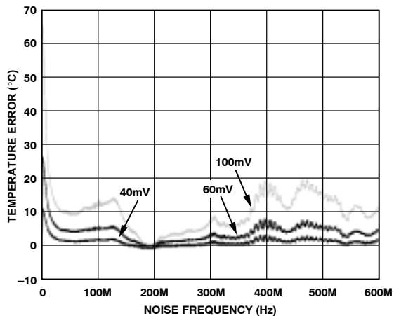
Figure 6. Remote Temperature Error vs. Differential-Mode Noise Frequency
