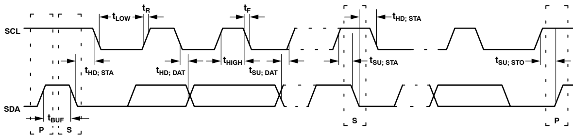
Figure 2. SMBus Bus Timing
