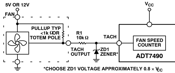
Figure 44. Fan with Strong TACH Pullup to >V CC or Totem-Pole Output, Clamped with Zener Diode and Resistor
