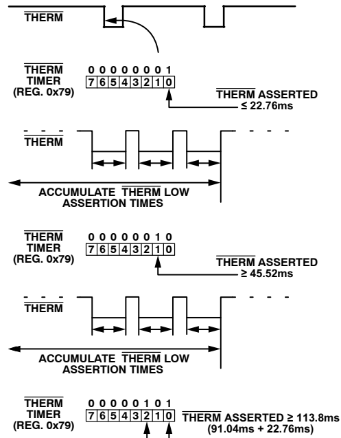
Figure 33. Understanding the THERM Timer
