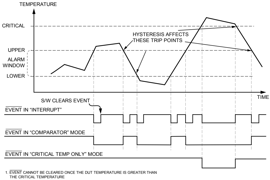
Figure 15. Hysteresis Detail
