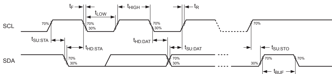
Figure 4. Bus Timing
