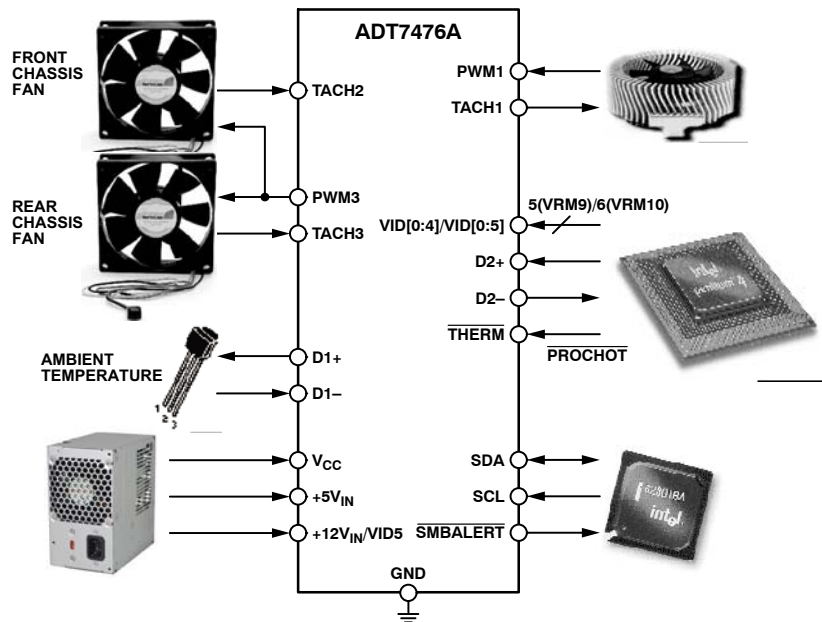
Figure 13. ADT7476A Configuration
