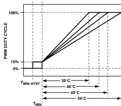
Figure 59. Increasing T_{\text{RANGE}} Changes the AFC Slope
