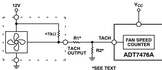
Figure 44. Fan with Strong TACH Pullup to >V CC or Totem-Pole Output, Attenuated with R1/R2
