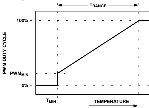
Figure 57. T_{\text{RANGE}} Parameter Affects Cooling Slope
