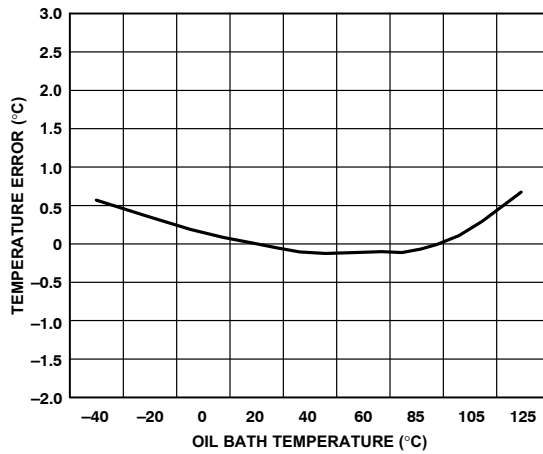
Figure 11. Remote Temperature Error vs. ADT7476A Temperature
