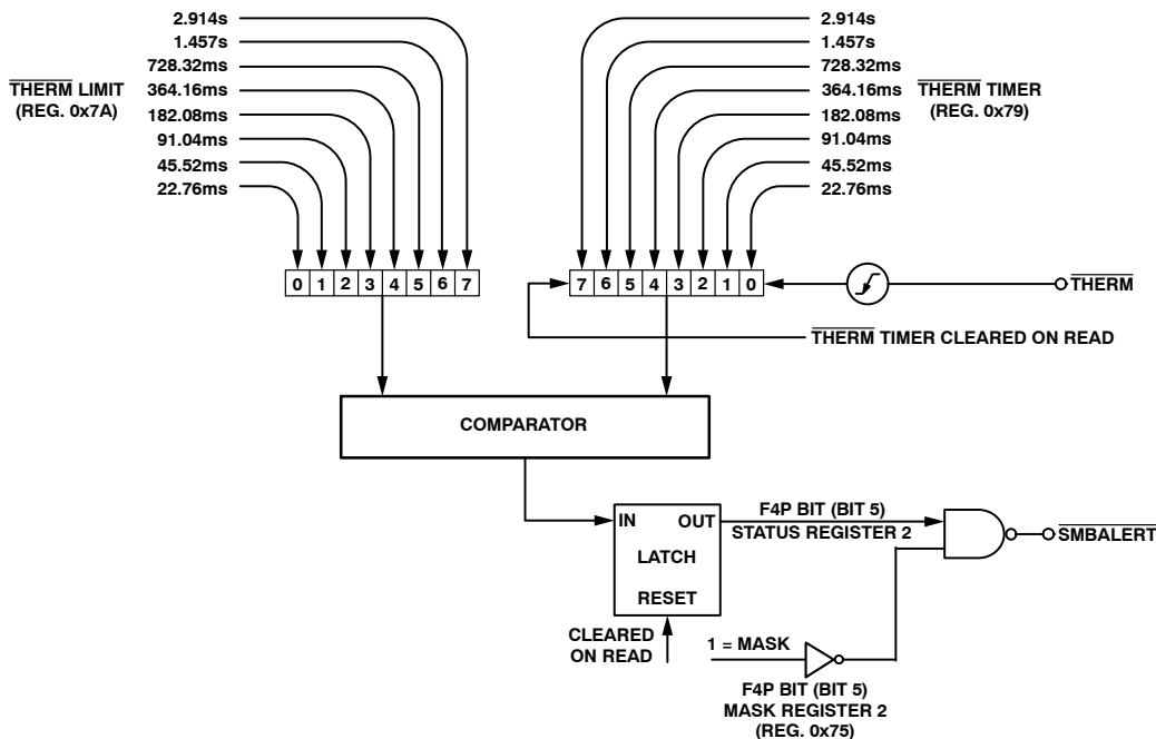
Figure 33. Functional Block Diagram of \overline{\text{THERM}} Monitoring Circuitry
