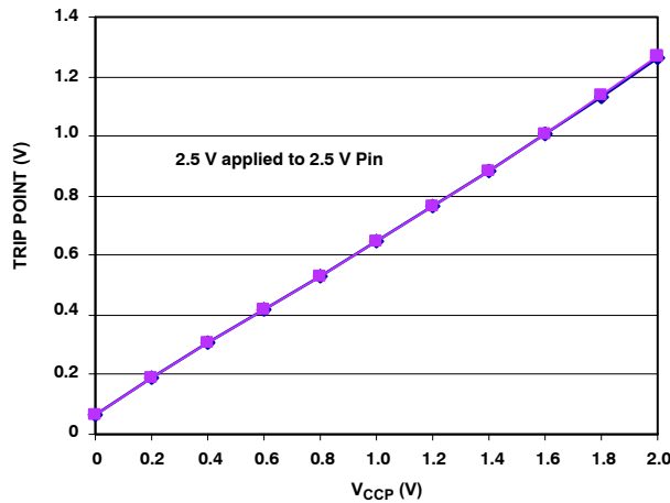
Figure 12. THERM Input Threshold vs. V CCP Voltage
