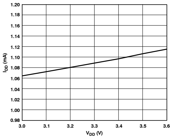
Figure 7. Normal I DD vs. Power Supply
