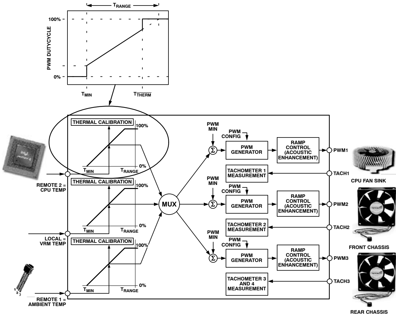
Figure 64. How T_{THERM} Relates to Automatic Fan Control
