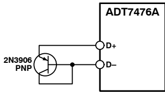
Figure 27. Measuring Temperature Using an PNP Transistor
