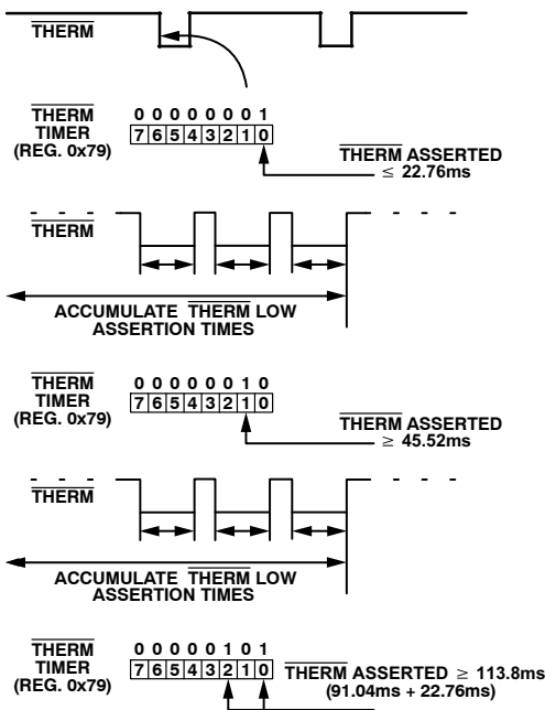
Figure 32. Understanding the \overline{\text{THERM}} Timer
