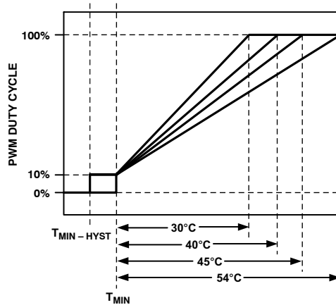
Figure 54. Increasing T RANGE Changes the AFC Slope
