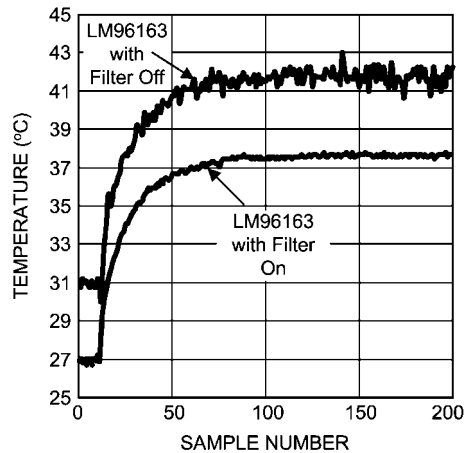
FIGURE 5. Digital Filter Response in a typical Intel processor on a 65 nm or 90 nm process. The filter curves were purposely offset for clarity.
