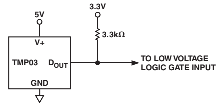
Figure 6. Interfacing to Low Voltage Logic
