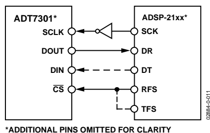
Figure 18. ADT7301-to-ADSP-21xx Interface
