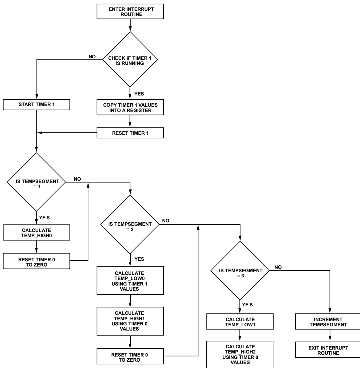
Figure 36. ADuC812 Interrupt Routine Flowchart
