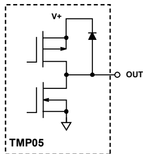
Figure 28. TMP05 Digital Output Structure
