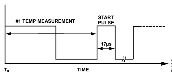
Figure 26. Daisy-Chain Temperature Measurement and Start Pulse Output from First TMP05/TMP06
