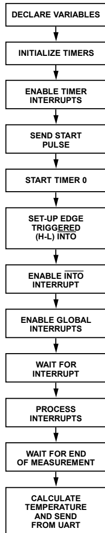
Figure 34. ADuC812 Main Routine Flowchart
