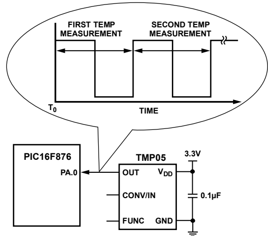
Figure 37. Typical Continuously Converting Application Circuit
