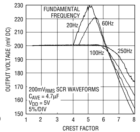
Performance vs Large Crest Factors
