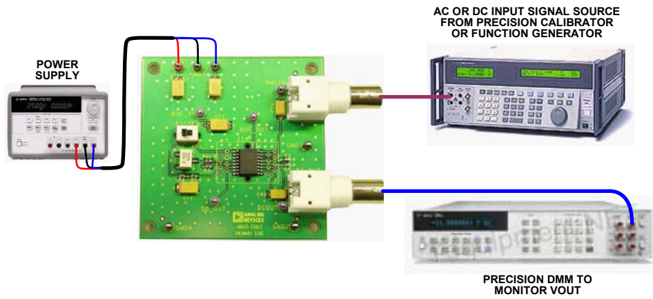
Figure 31. AD637-EVALZ Typical Bench Configuration
