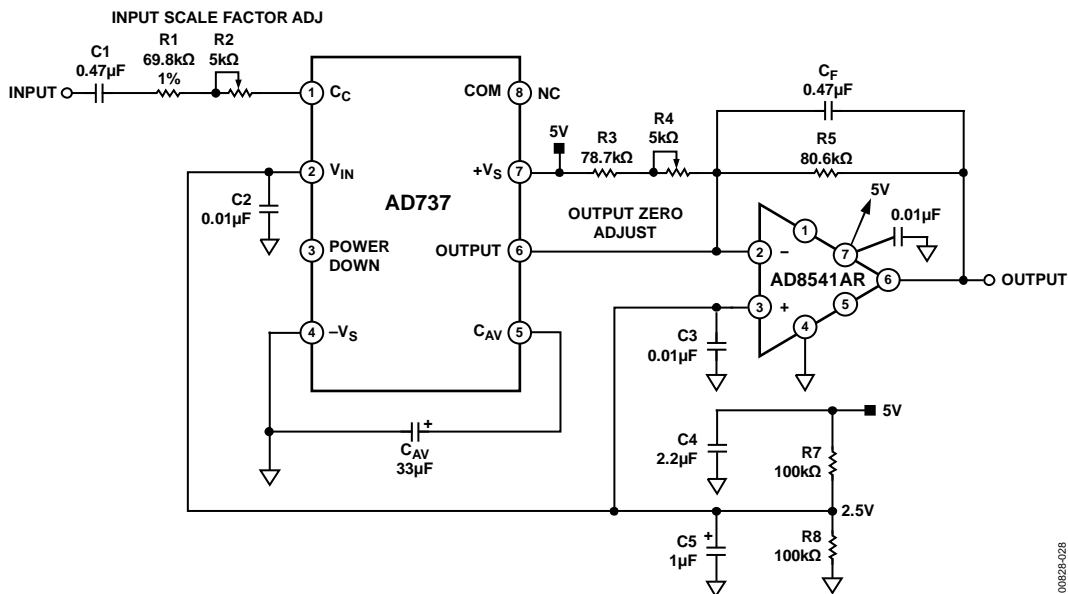
Figure 29. Battery-Powered Operation for 200 mV Maximum RMS Full-Scale Input
