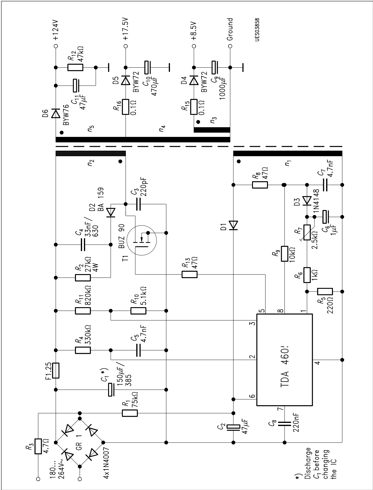
Application Circuit
