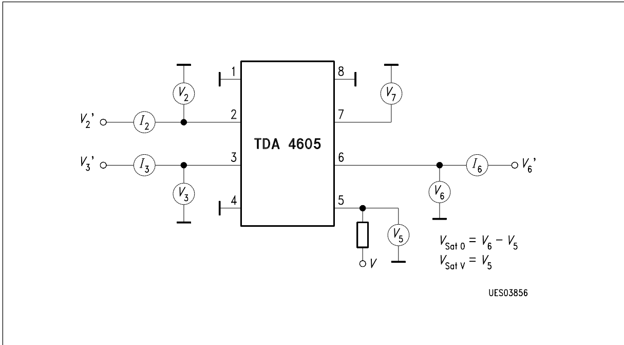
Test Circuit 1
