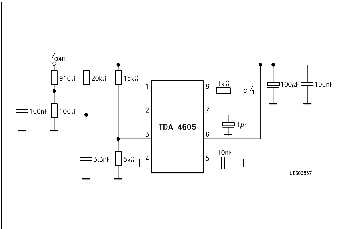
Test Circuit 2
