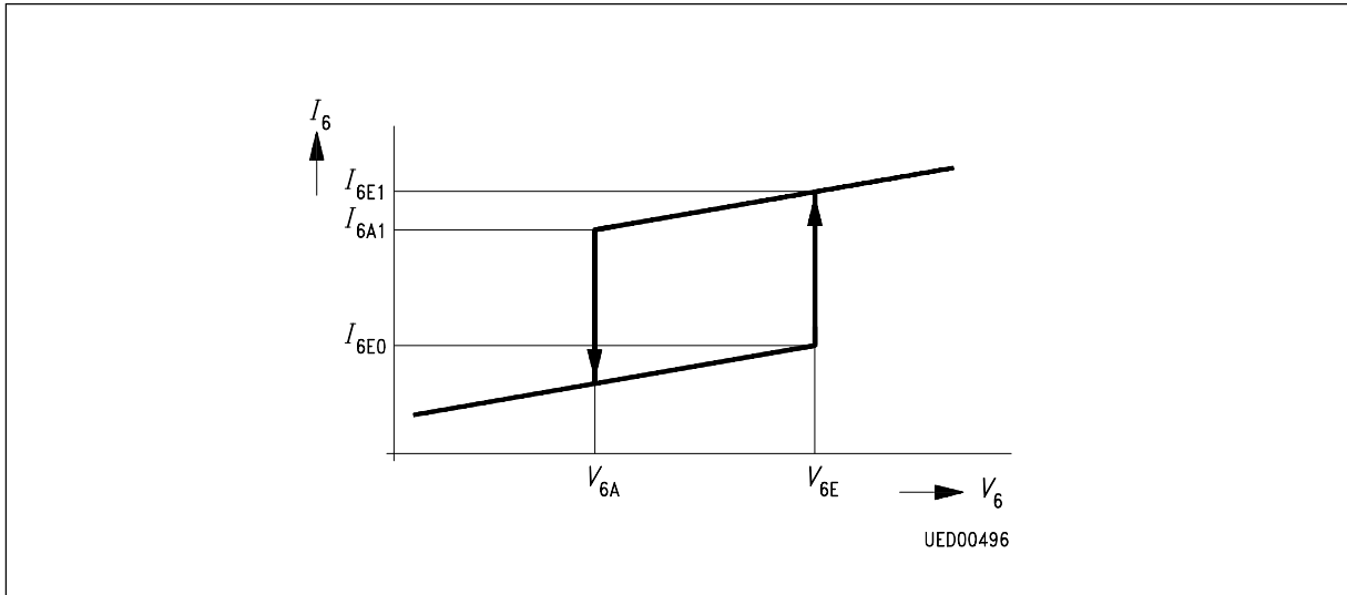
Start-Up Hysteresis
