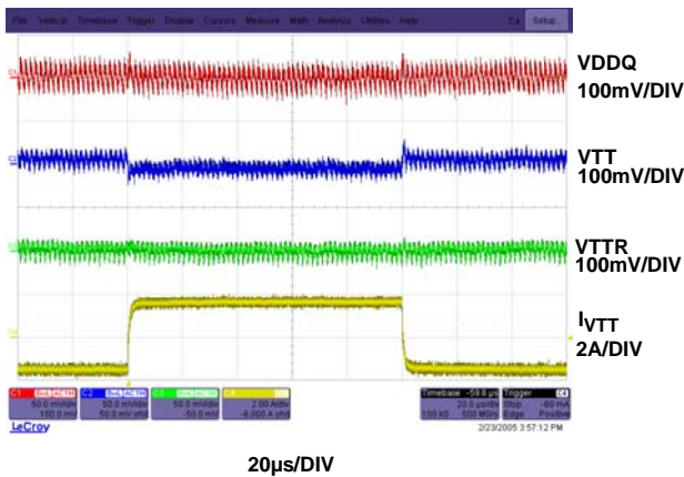
FIGURE 11. LOAD TRANSIENT (VTT -1.5A TO 1.5A)
