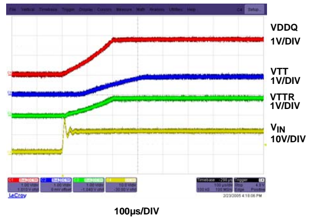
FIGURE 12. POWER-UP WAVEFORMS
