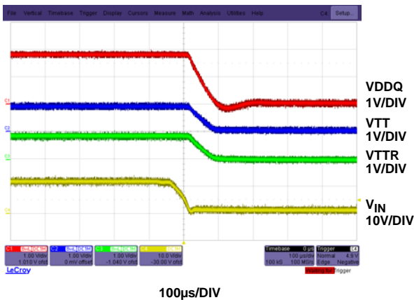
FIGURE 13. POWER-DOWN WAVEFORMS
