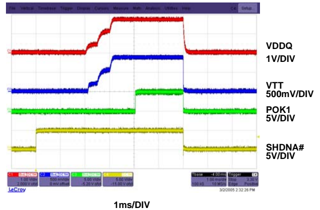
FIGURE 14. VDDQ START-UP AND SHUTDOWN INTO HEAVY LOAD, DISCHARGE DISABLED
