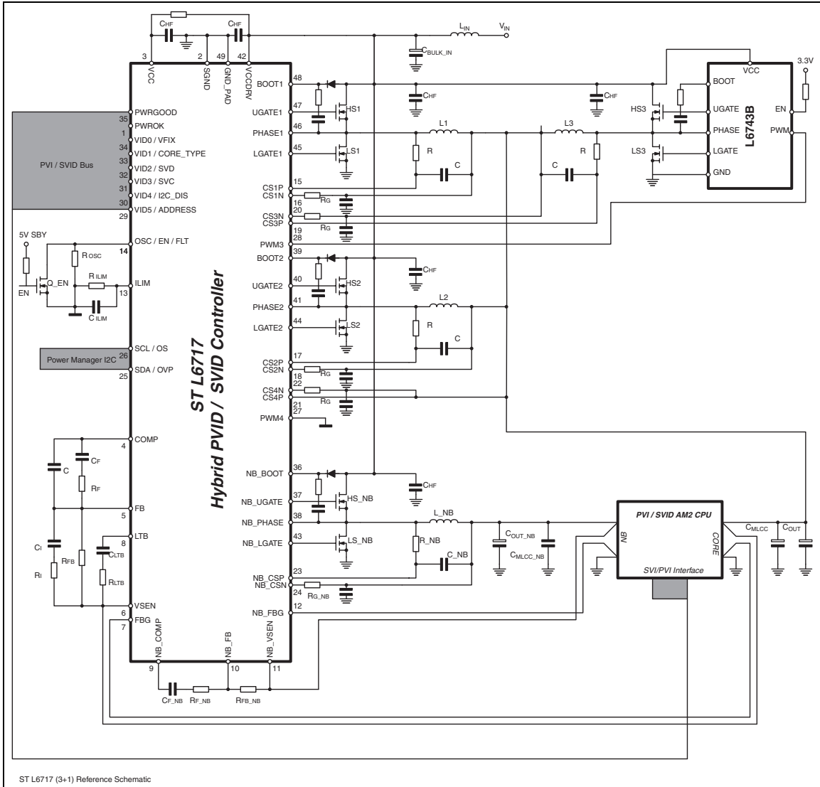
Figure 2. Typical 3+1 application circuit
