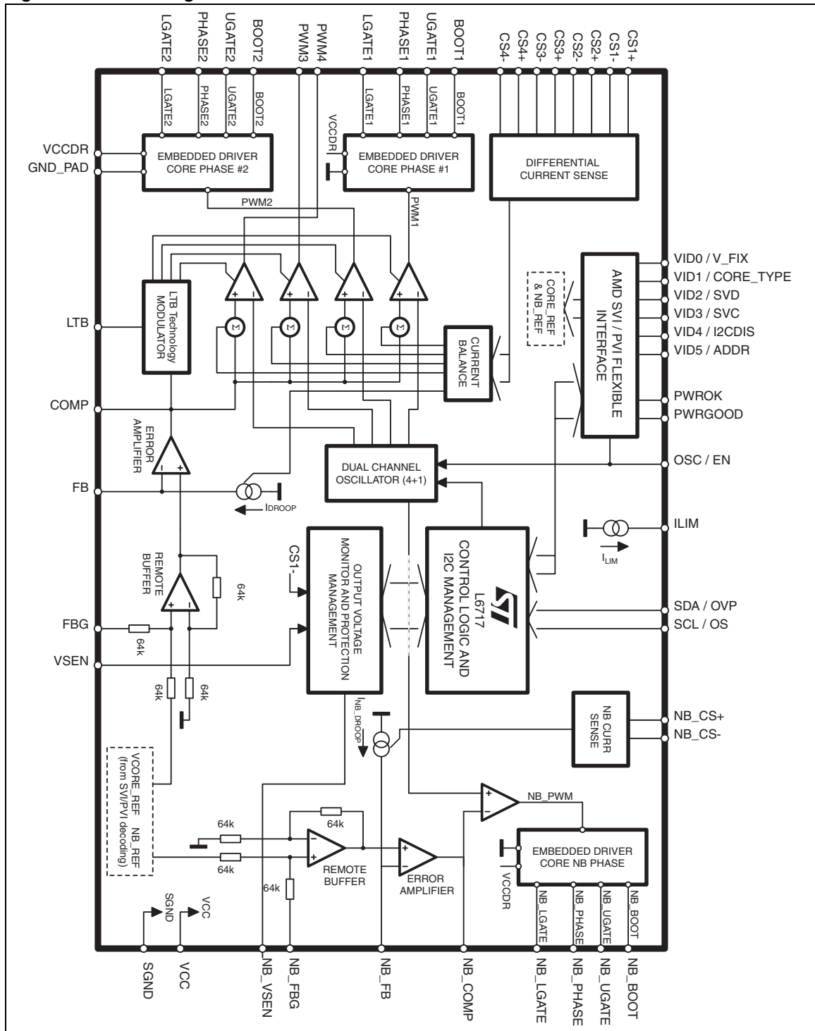
Figure 4. Block diagram
