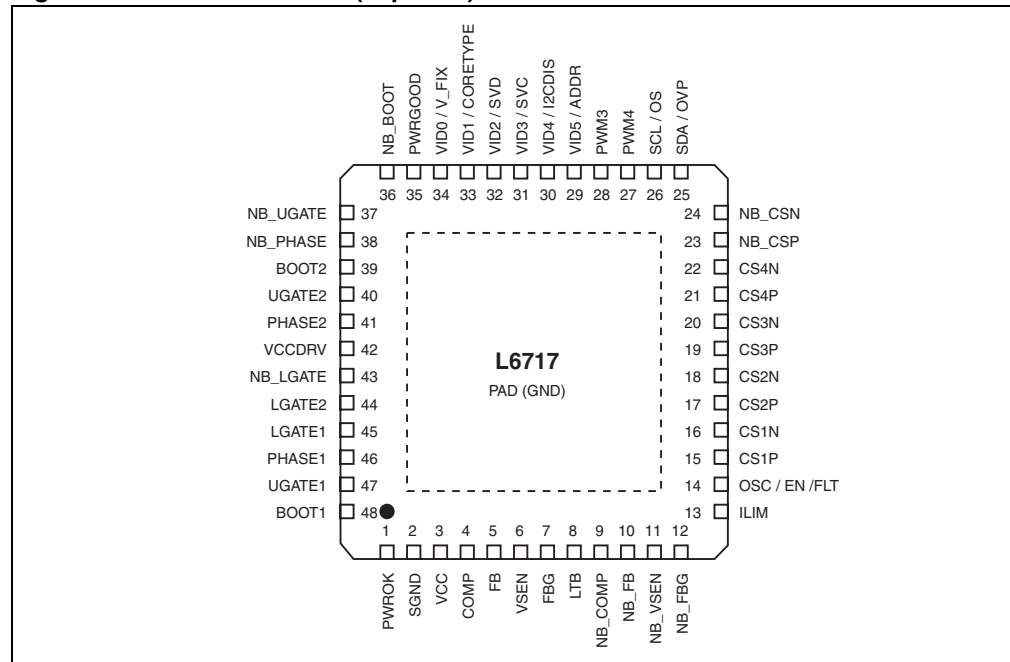
Figure 5. Pins connection (Top view)
