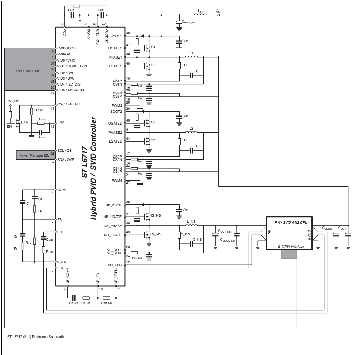
Figure 3. Typical 2+1 application circuit
