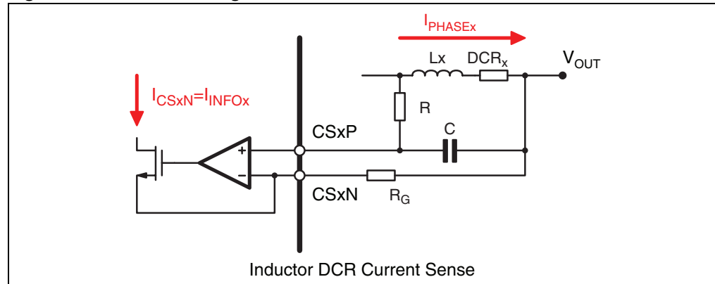
Figure 10. Current reading
