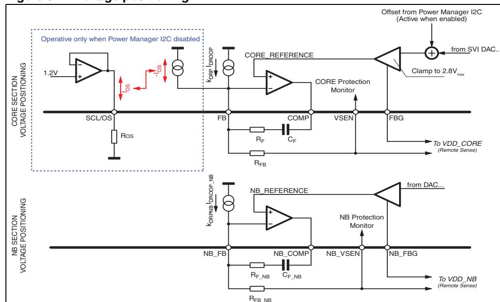
Figure 9. Voltage positioning
