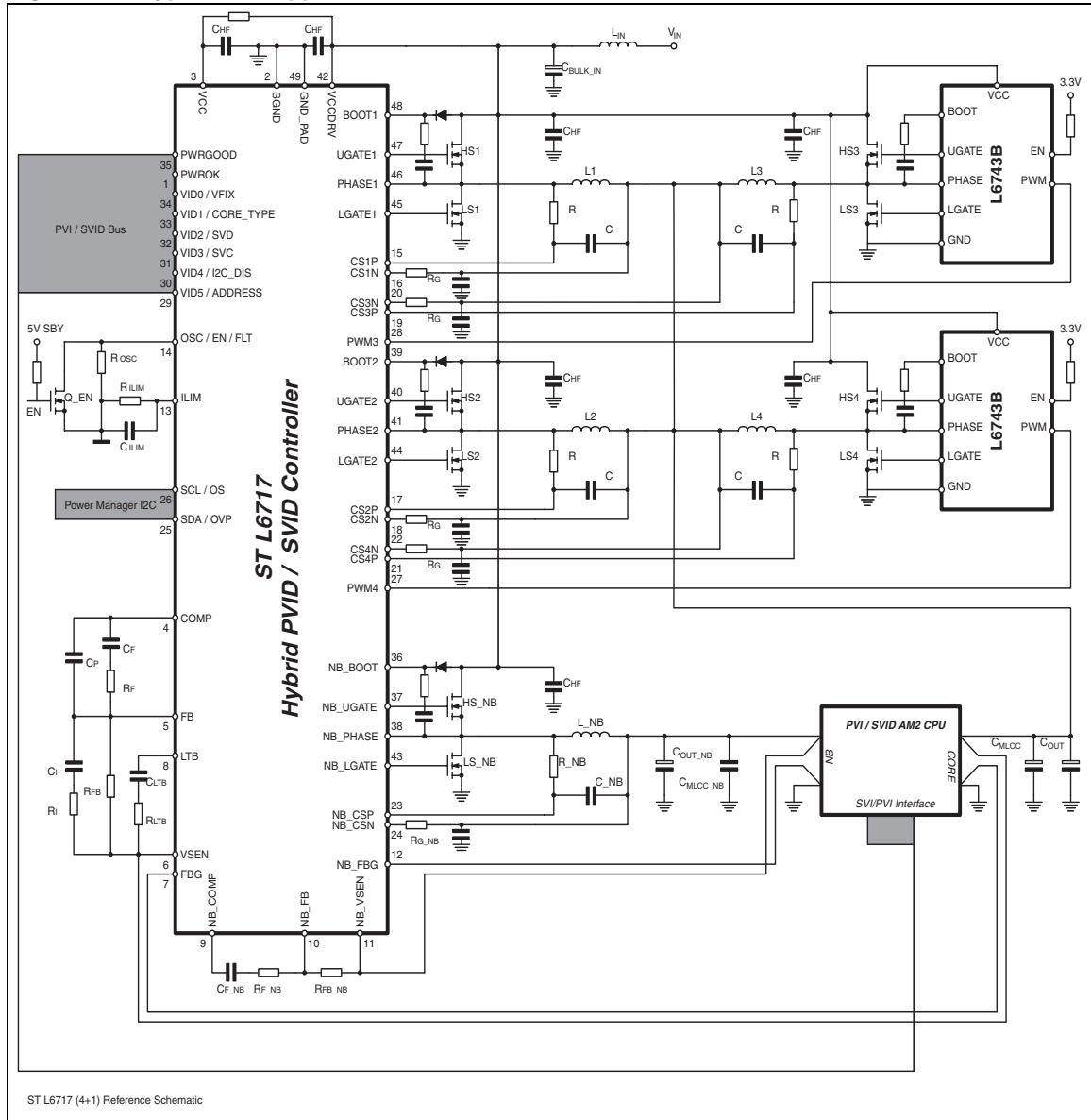
Figure 1. Typical 4+1 application circuit
