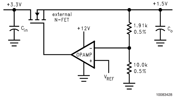
FIGURE 9. V_{\text{REF}} Used in an N-FET LDO Supply
