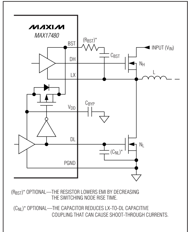
Figure 11. Gate-Drive Circuit
