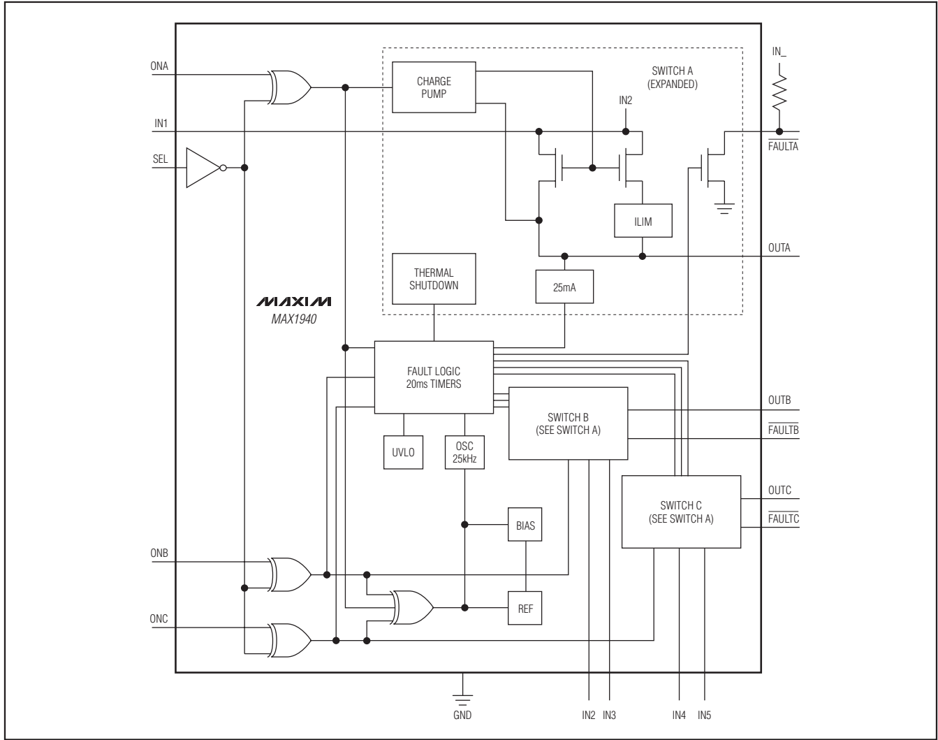
Figure 1. Functional Diagram
