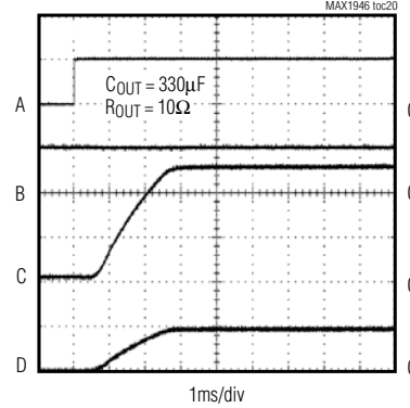
STARTUP WAVEFORMS C_{OUT} = 330\mu F
