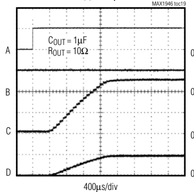
STARTUP WAVEFORMS C_{OUT} = 1\mu F
