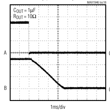
SWITCH TURN-OFF TIME ( t_{OFF} + t_{FALL} )
