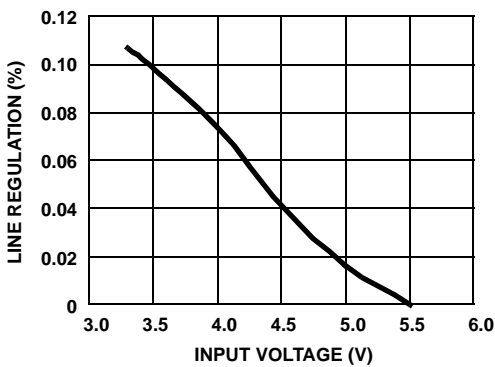
FIGURE 5. BOOST LINE REGULATION vs INPUT VOLTAGE (PI-MODE)
