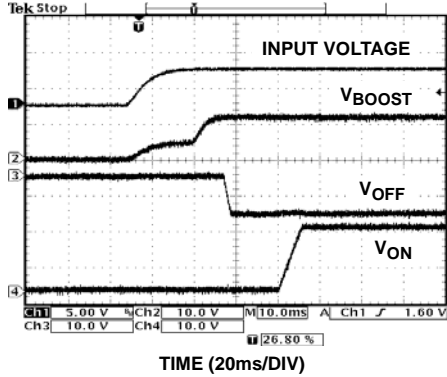
FIGURE 13. START-UP SEQUENCE
