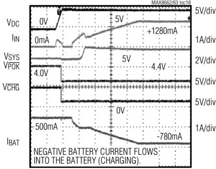
400 \mu s /div PEN1 = PEN2 = 1, \overline{CEN} = 0 , VBAT = 4.0V, I_{SYS} = 500mA , EN_ = 1
