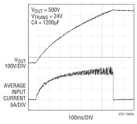
Charging Waveform
