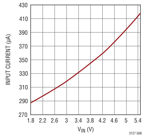
Quiescent Current vs V_{IN} (Fixed Frequency Mode—Not Switching)
